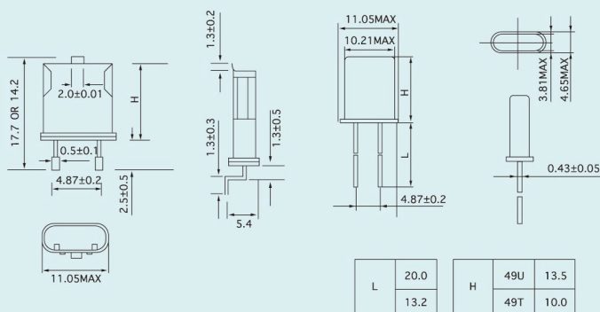
49U/49T DIMENSIONS(mm)
