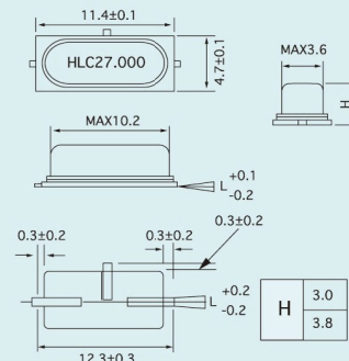
49S/SMD3L DIMENSIONS(mm)
