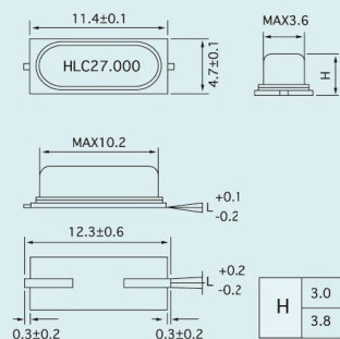
49S/SMD DIMENSIONS(mm)
