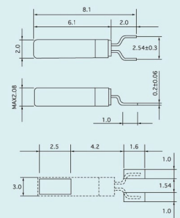
PMX-206S DIMENSIONS (mm)
