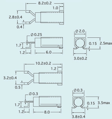
PMX-308FA, PMX-206FA DIMENSIONS (mm)
